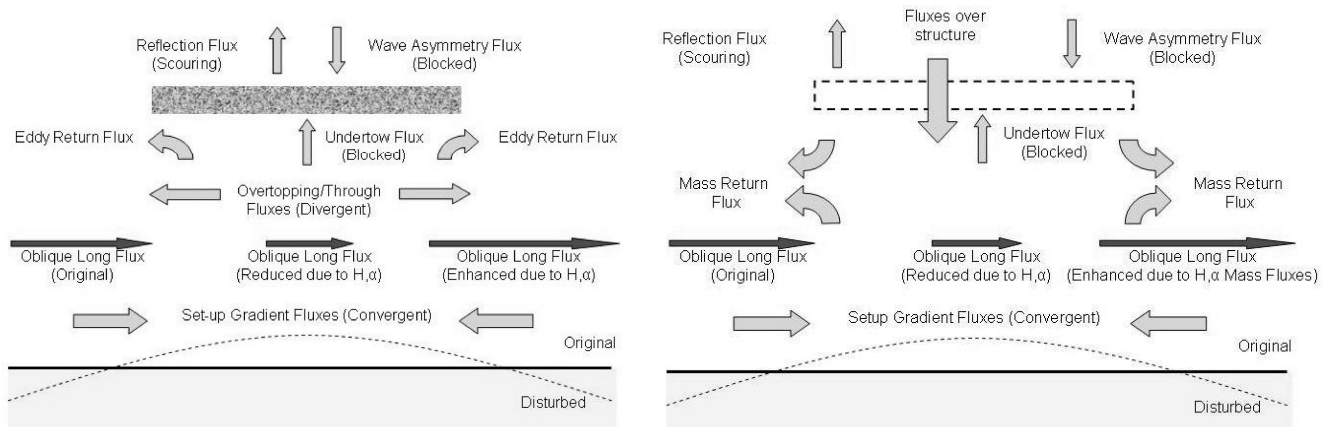
Figure 37 Shore-parallel detached breakwaters
