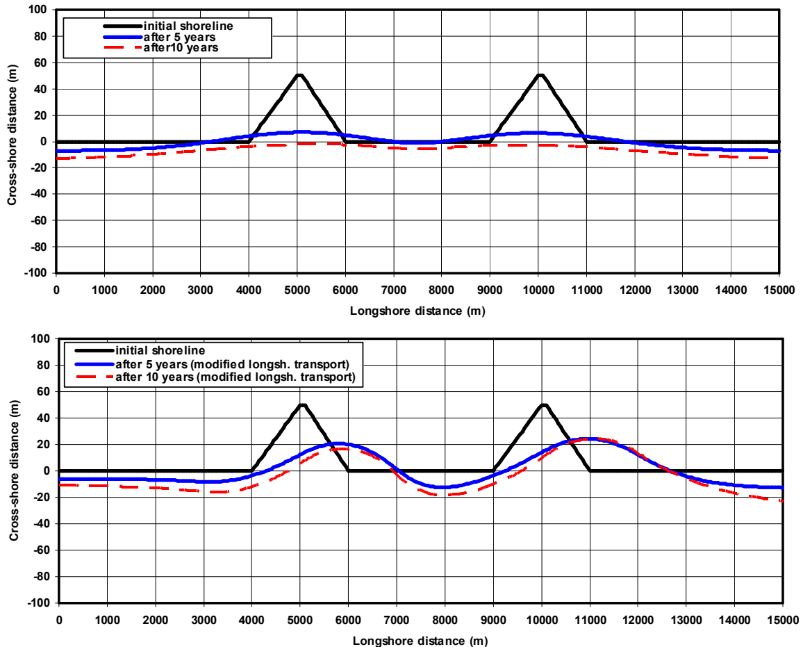
Figure 19 Shoreline behaviour after 5 and 10 years of headland-type beach fills (net longshore transport from left to right); spacing of 5000 m. Top: standard longshore transport Bottom: longshore transport on updrift flank is 20% larger than on downdrift flank of headland
