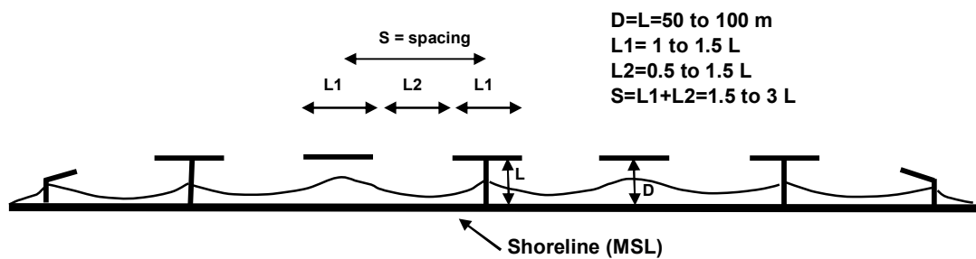
Figure 46 Coastal protection by T-head groynes and detached breakwaters
