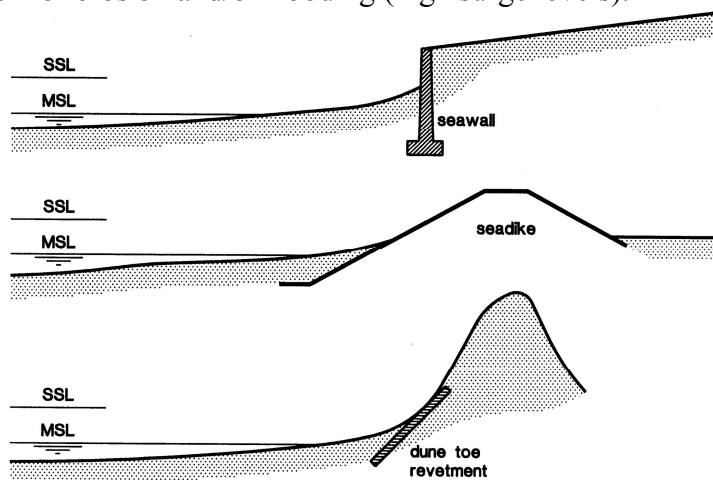
Figure 25 Seawall, seawall and revetment
