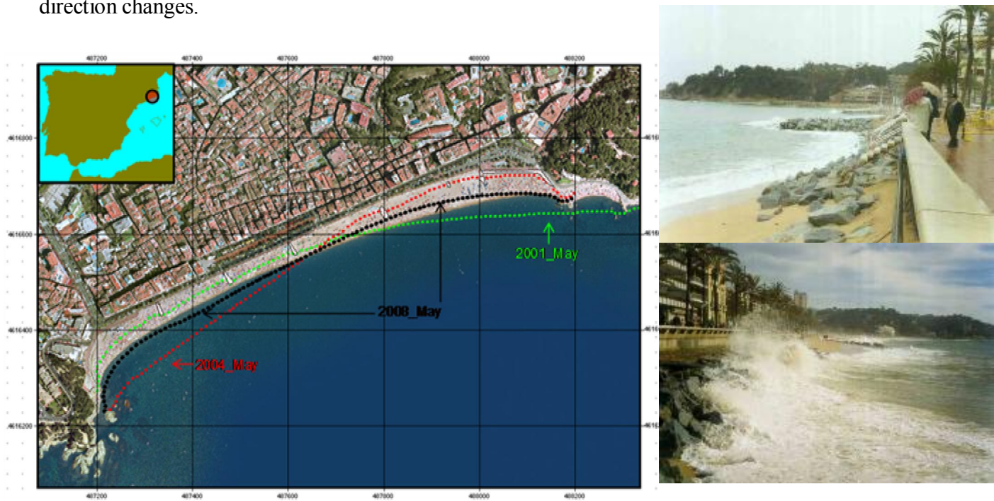
Figure 33 Beach rotation (May 2001, 2004 and 2008) and storm impact at Lloret de Mar, Spain
