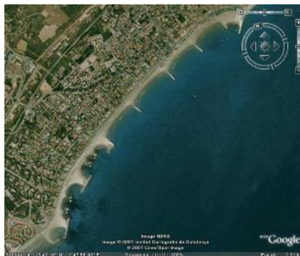
Figure 40 Coastal protection by various hard structures at beach of Sitges, south of Barcelona, Spain
