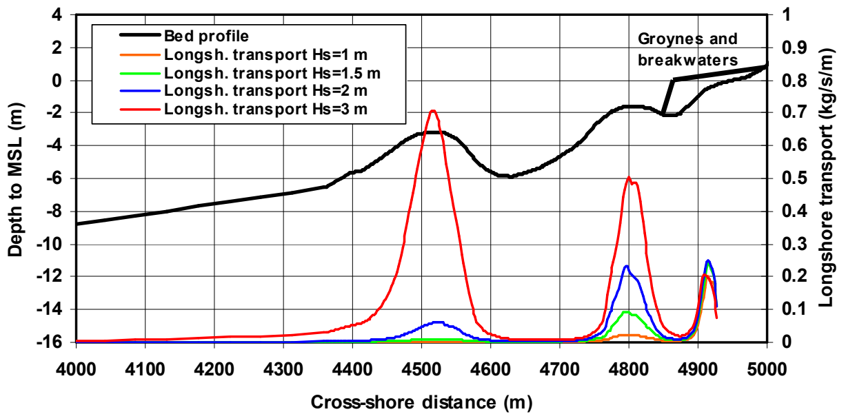
Figure 47 Cross-shore distribution of longshore transport for offshore wave heights of 1 to 3 m; offshore wave incidence angle of 30° and d_{50}=0.2 mm (sand)
