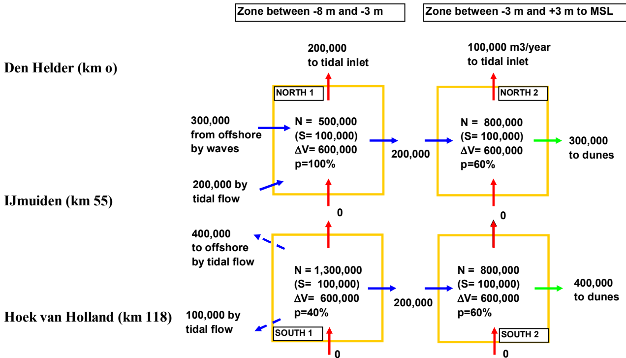
Figure 24 Sediment budget for subcells of Holland coast; period 1990 to 2006 (15 years) N = nourishment volume (m 3 /year); ΔV = measured volume increase (m 3 /year), S = compensation volume related sea level rise (m 3 /year), p =over-nourishment percentage (in %)
