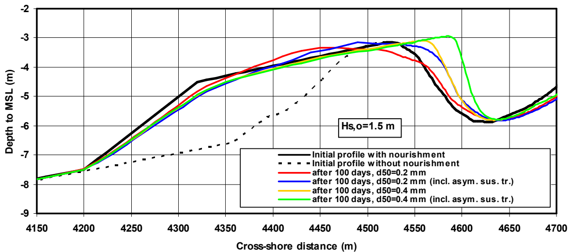
Figure 17 Onshore migration of shoreface nourishment; H_{s,o}=1.5 \text{ m} , sediment d_{50}=0.2 \text{ mm} and 0.4 \text{ mm}
