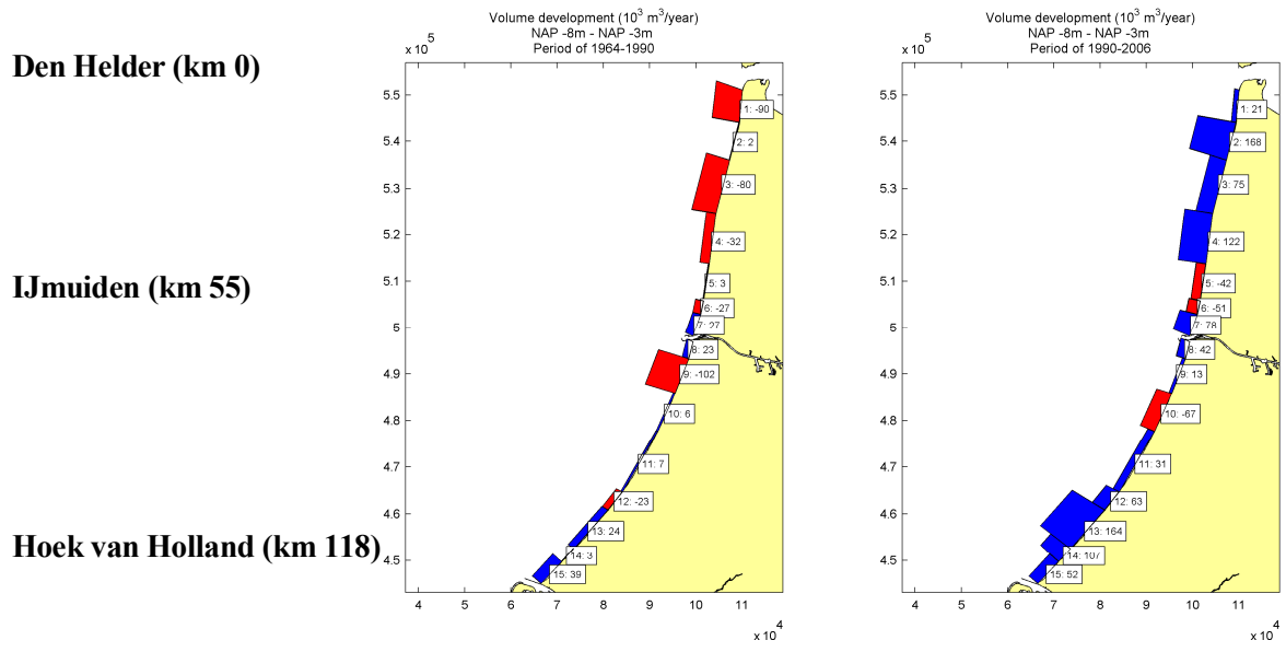
Figure 21 Volume changes in zone between -8 m and -3 m (to MSL) depth contours (Red=erosion volume, -90,000 m^3 in Section 1; Blue=deposition volume, 21,000 m^3 in Section 1) Left: period 1964 to 1990 Right: period 1990 to 2006
