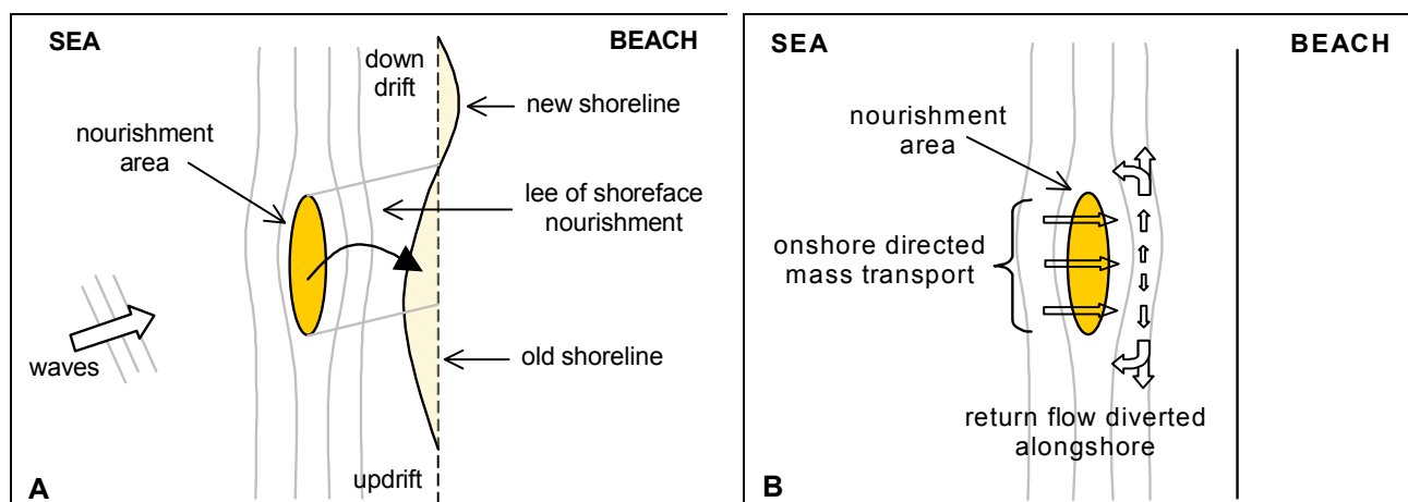
Figure 7 Effects of a shoreface nourishment
