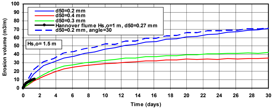
Figure 14 Cumulative erosion of beach nourishments; H_{s,o} = 1.5 m; sediment d_{50} = 0.2, 0.3 and 0.4 mm
