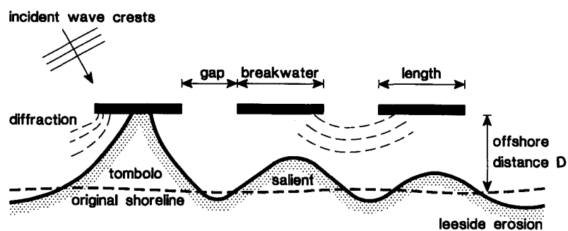
Figure 37 Shore-parallel detached breakwaters
