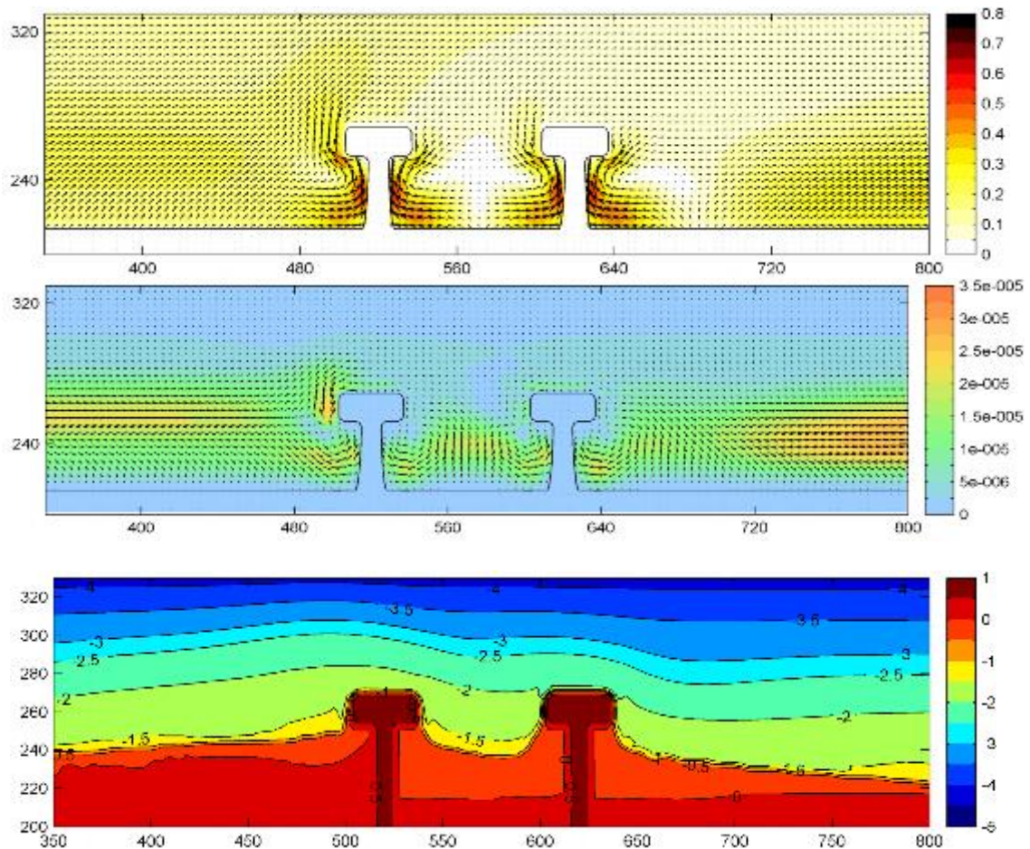
Figure 36 Computed results for T-head groynes along coast of Turkey (longshore current and transport from left to right →) Top: depth-averaged velocity vectors Middle: transport vectors (in m^2/s ) Bottom: bathymetry after 15 days (in m)
