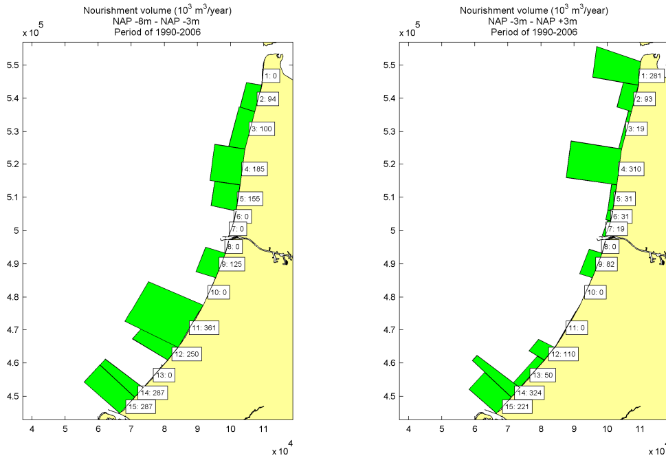
Figure 23 Nourishment volumes in period 1990 to 2006 Left: zone between -8 and -3 m depth contours Right: zone between -3 and +3 m depth contours
