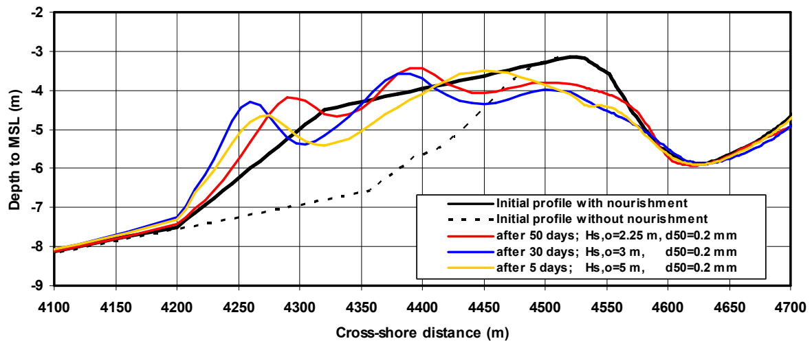
Figure 18 Offshore migration of shoreface nourishment; H_{s,o}=2.25 to 5 \text{ m} , sediment d_{50}=0.2 \text{ mm}
