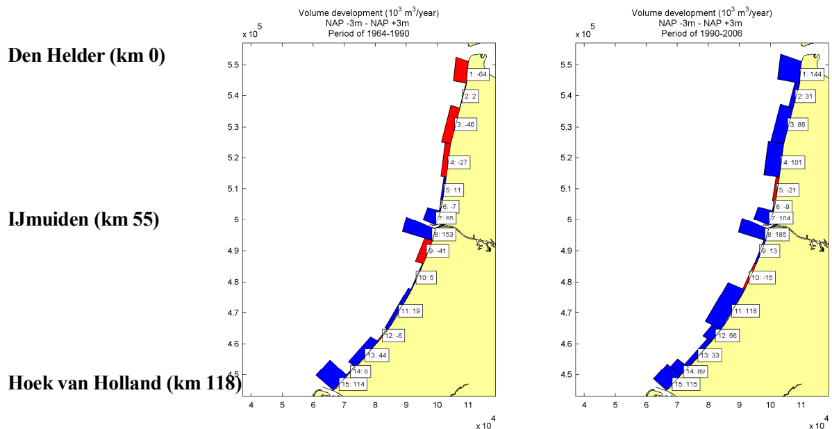
Figure 22 Volume changes in zone between -3 m and +3 m (to MSL) depth contours (Red=erosion volume, -64,000 m^3 in Section 1; Blue=deposition volume, 144,000 m^3 in Section 1) Left: period 1964 to 1990 Right: period 1990 to 2006
