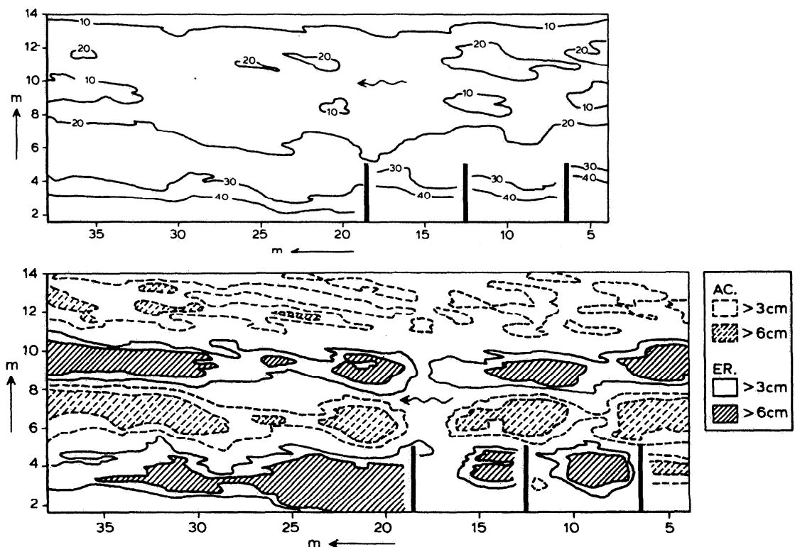
Figure 27 Effect of groynes on coast, Test T23 (Hulsbergen et al., 1977) (longshore drift from right to left; 0= updrift; 35 m= downdrift) Top: contour lines (in cm above bottom of basin) after 50 hours Bottom: bed level changes in cm after 50 hours (AC. = accretion; ER. = erosion)
